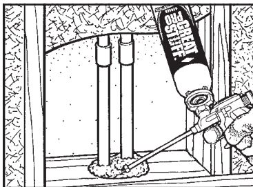
Electrical wire penetration
